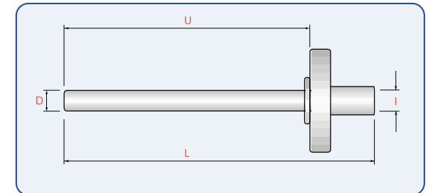
Fabricated thermowell with process flange and extension piece.
