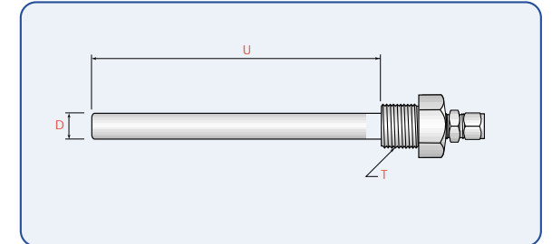
Fabricated Thermowell with parallel male process connector and compression fitting.
