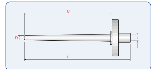
Solid drilled tapered thermowell with process flange and lagging extension.
